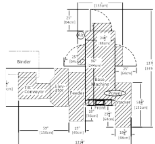
IN-LINE WITH PILE FEEDER
